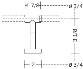
wide bracket
