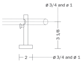
rest-in bracket
