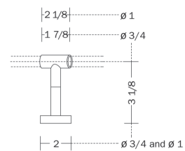
plug-in bracket
