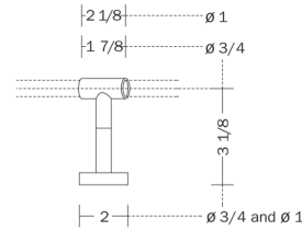
wide bracket
