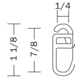
pleating hook
