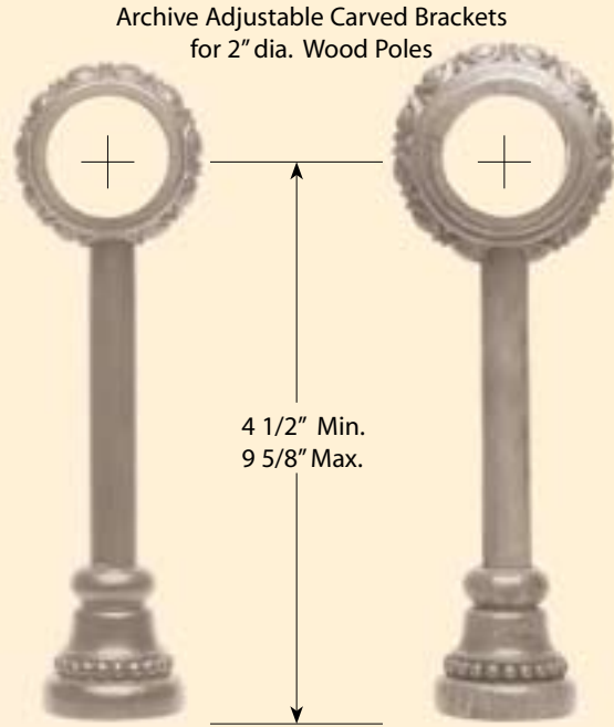
AR40 Proj.: 11 3/8" - W: 3 1/8" Base L: 2 1/2" - Dia.: 2 5/8" Finishes: CLA, OLD, OXF
